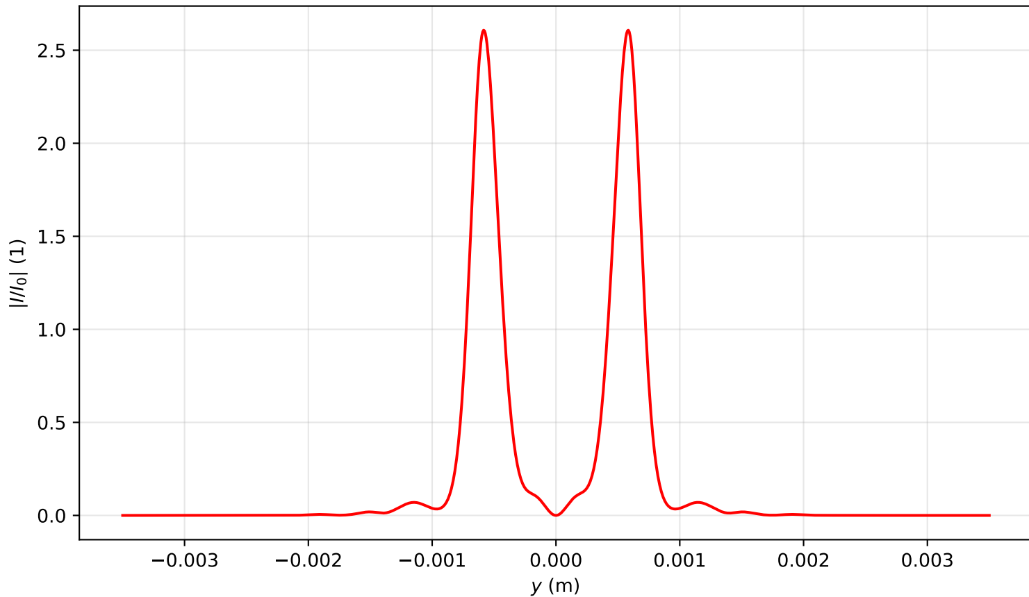
Intensity profile I(x=0, y, z=1.035)/I_0 , P_{in}=9.0P_{cr} , artificial time
